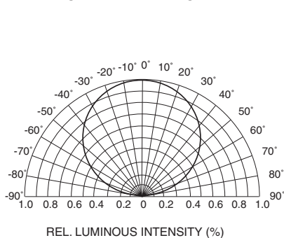
Fig.4 Radiation Diagram
