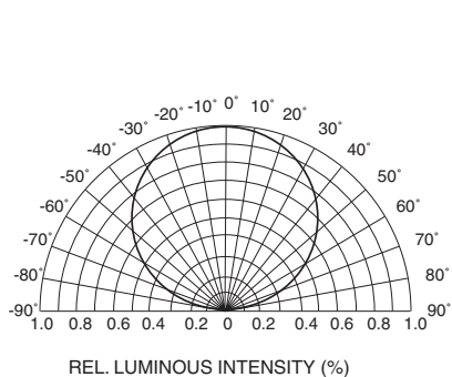
Fig.4 Radiation Diagram
