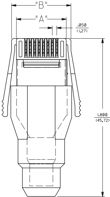
KEYING OPTION "1"
