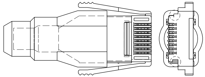
KEYING OPTION "2"
