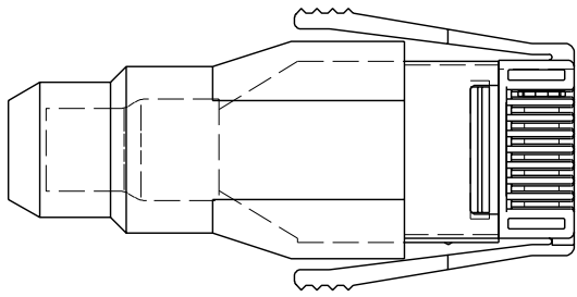
KEYING OPTION "1"
