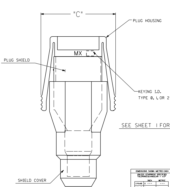
KEYING OPTION "2"
