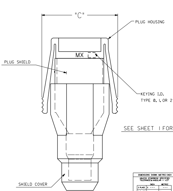
KEYING OPTION "2"
