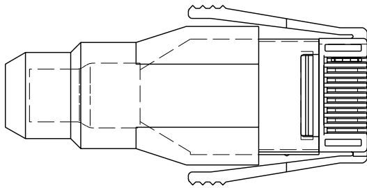
KEYING OPTION "1"
