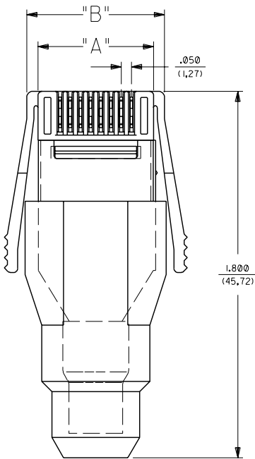
KEYING OPTION "1"
