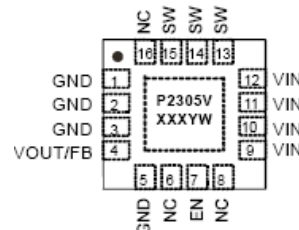
Top View QFN 3x3 16L
