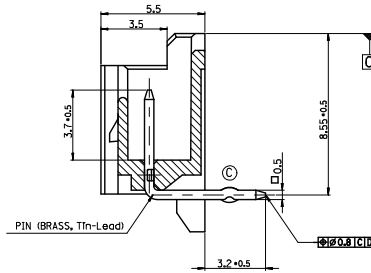
SECTION K-K'
