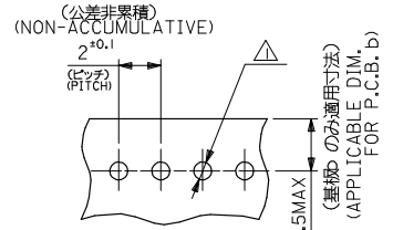
基板取付穴推奨寸法 RECOMMENDED P.C. BOARD HOLE DIM.
