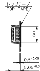
SECT. Z-Z
