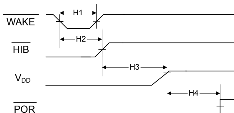
Figure 22-15. Hibernation Module Timing
