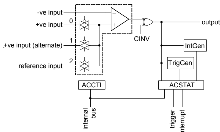
Figure 19-2. Structure of Comparator Unit
