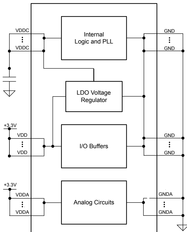
Figure 5-4. Power Architecture
