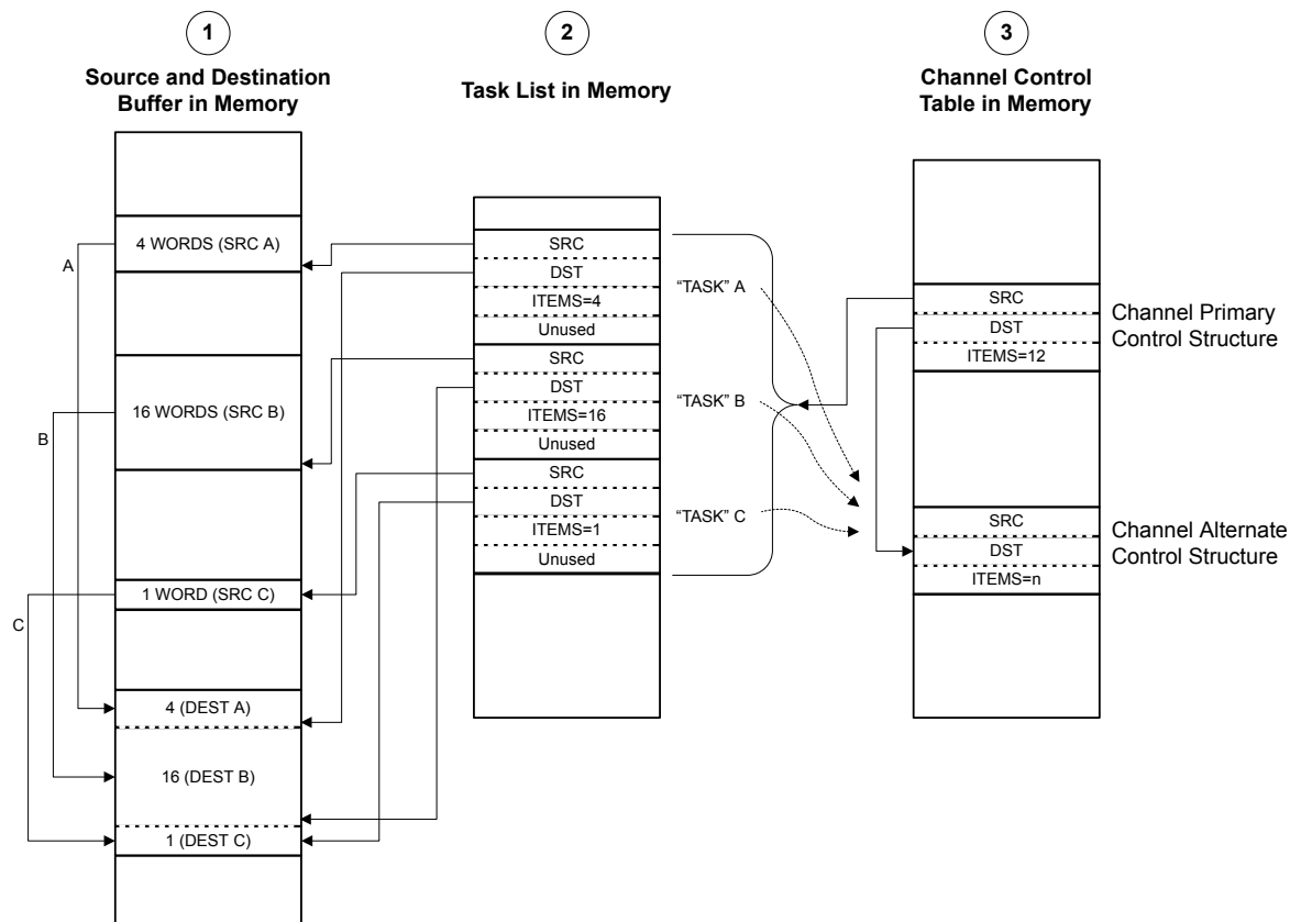
Figure 9-3. Memory Scatter-Gather, Setup and Configuration
