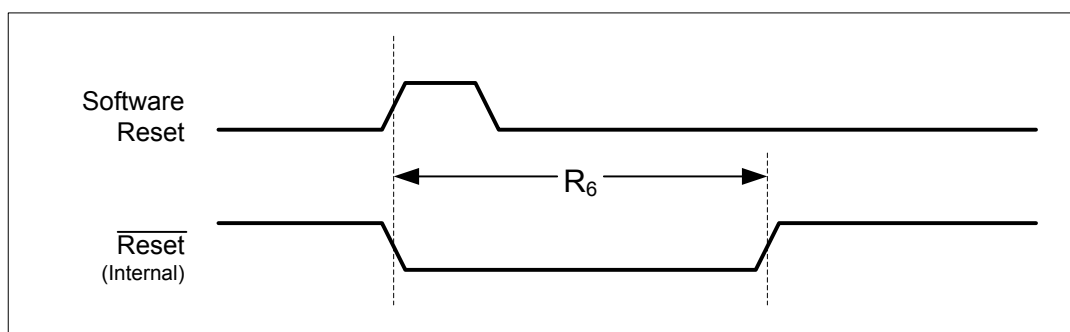
Figure 22-12. Software Reset Timing
