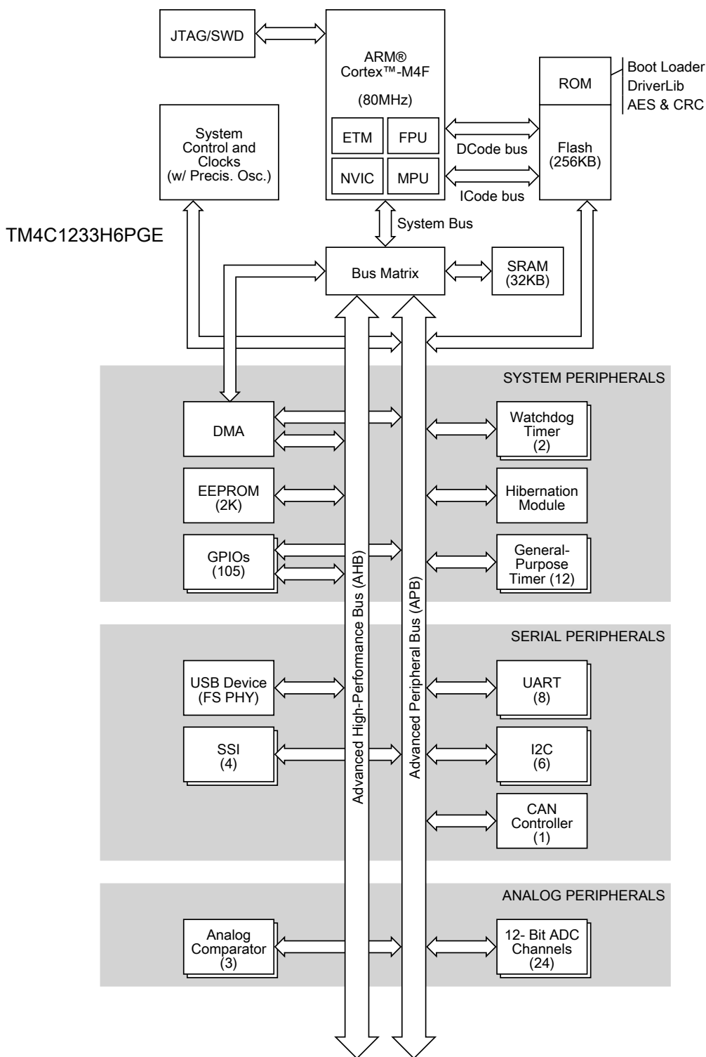
Figure 1-1. Tiva™ TM4C1233H6PGE Microcontroller High-Level Block Diagram
