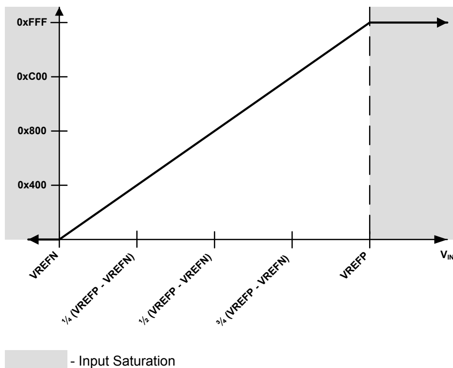
Figure 13-9. ADC Conversion Result
