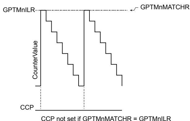
Figure 11-7. CCP Output, GPTMTnMATCHR = GPTMTnILR
