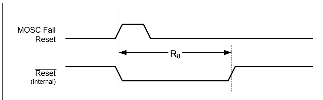
Figure 22-14. MOSC Failure Reset Timing
