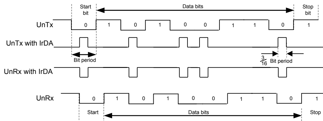
Figure 14-3. IrDA Data Modulation
