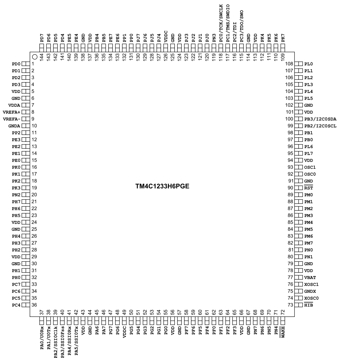
Figure 20-1. 144-Pin LQFP Package Pin Diagram
