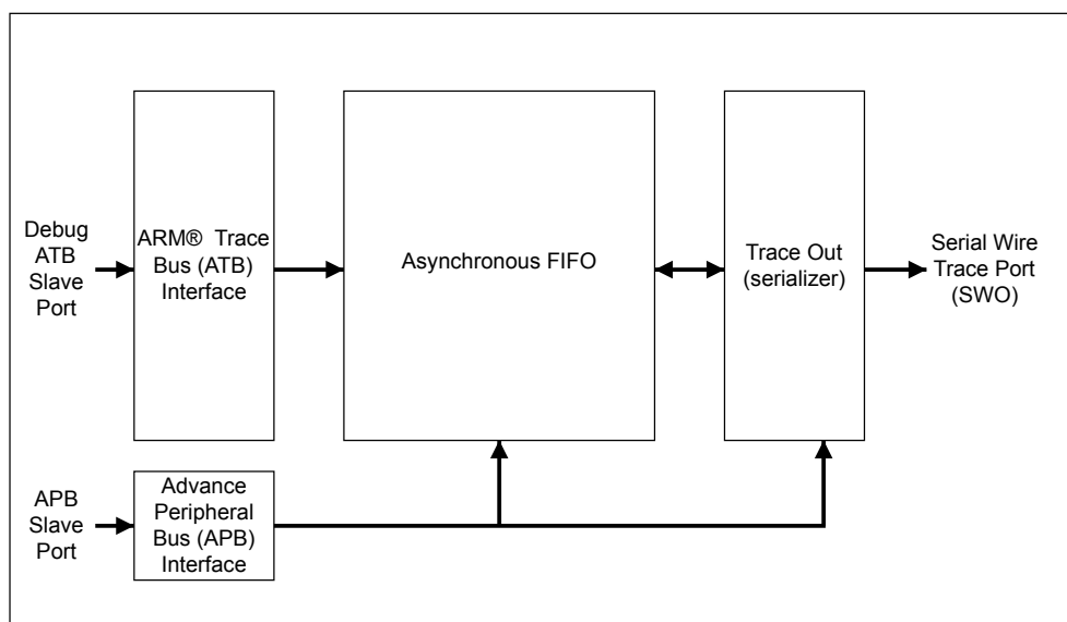
Figure 2-2. TPIU Block Diagram
