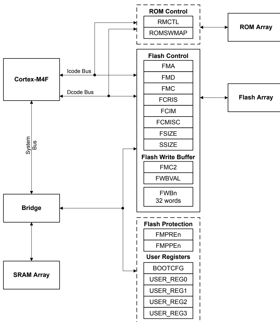
Figure 8-1. Internal Memory Block Diagram
