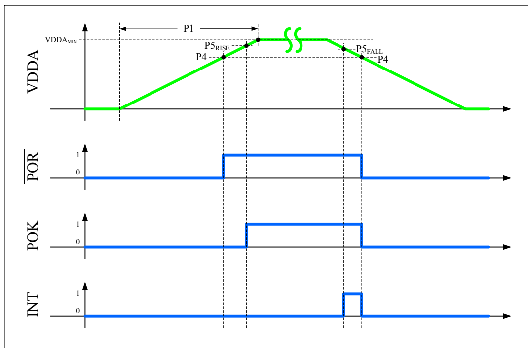
Figure 22-4. Power Assertions versus VDDA Levels
