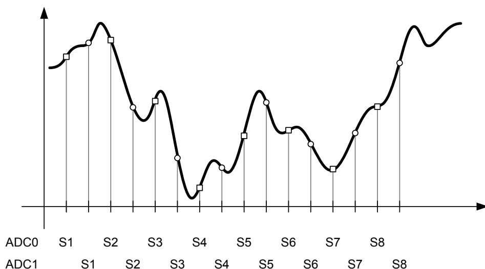
Figure 13-5. Skewed Sampling
