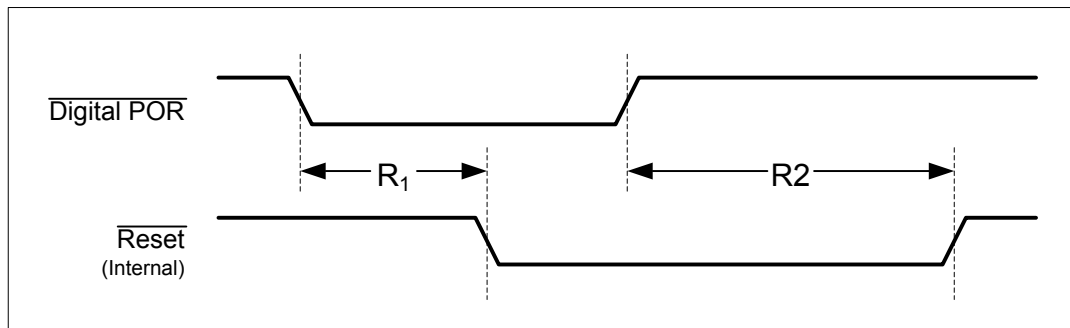
Figure 22-9. Digital Power-On Reset Timing
