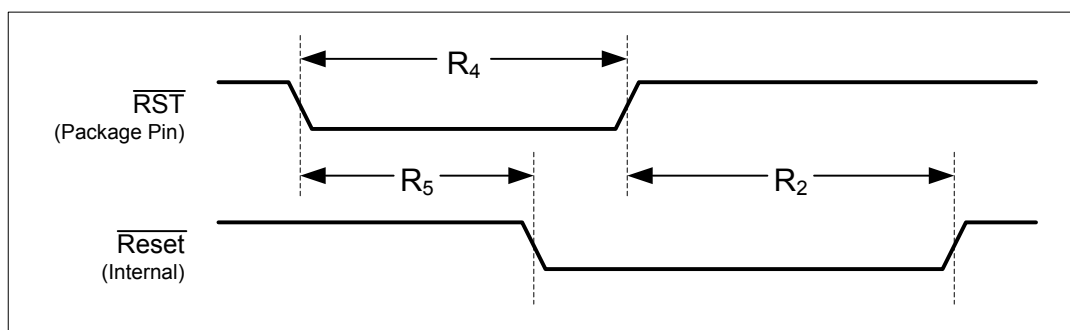
Figure 22-11. External Reset Timing ( \overline{RST} )
