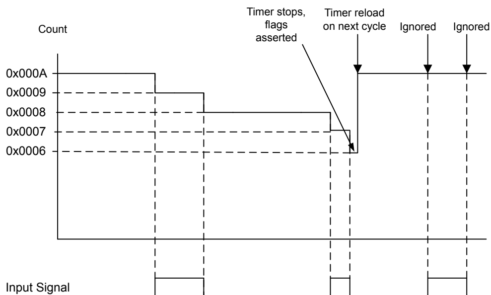
Figure 11-3. Input Edge-Count Mode Example, Counting Down
