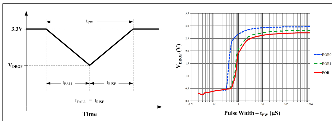
Figure 22-7. POR-BOR0-BOR1 VDD Glitch Response
