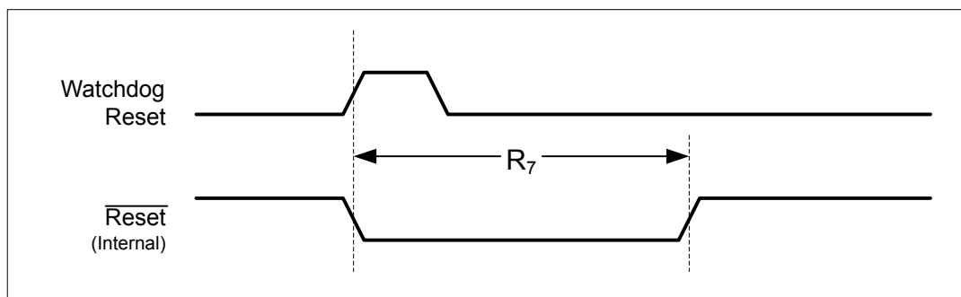
Figure 22-13. Watchdog Reset Timing
