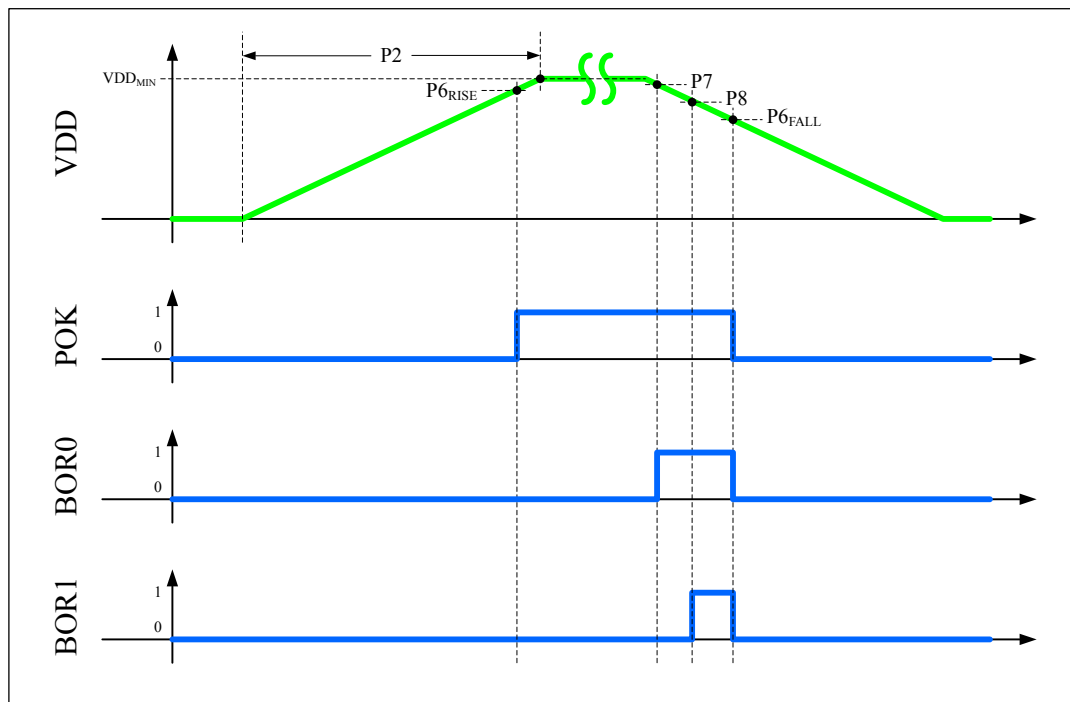
Figure 22-5. Power and Brown-Out Assertions versus VDD Levels
