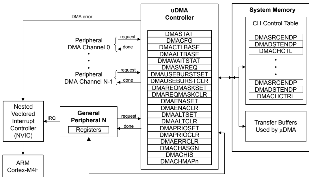
Figure 9-1. \mu DMA Block Diagram
