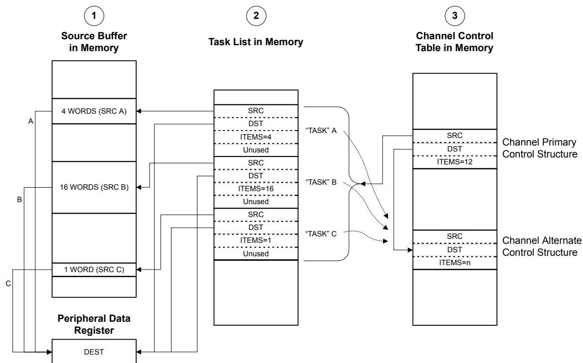
Figure 9-5. Peripheral Scatter-Gather, Setup and Configuration
