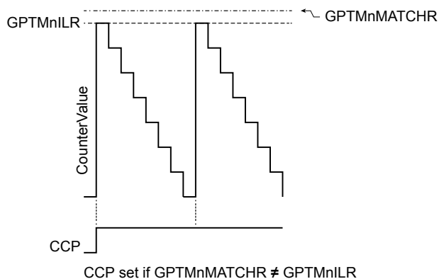
Figure 11-6. CCP Output, GPTMTnMATCHR > GPTMTnILR
