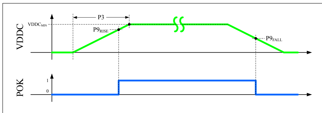
Figure 22-6. POK assertion vs VDDC
