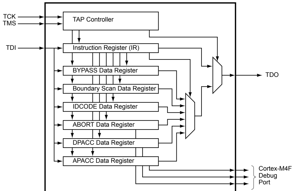
Figure 4-1. JTAG Module Block Diagram
