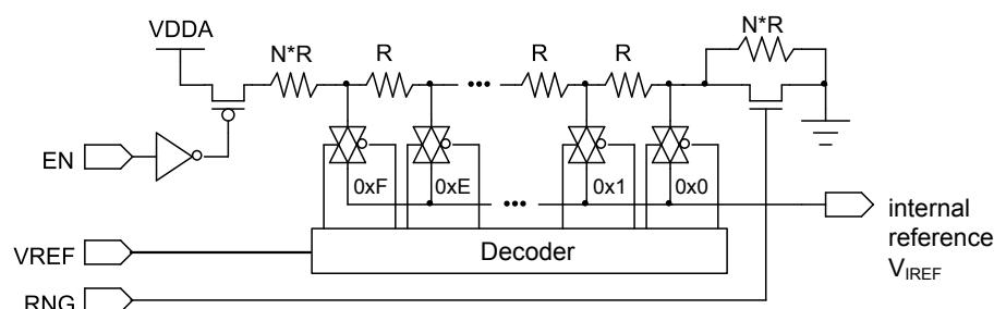
Figure 19-3. Comparator Internal Reference Structure
