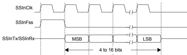
Figure 15-2. TI Synchronous Serial Frame Format (Single Transfer)
