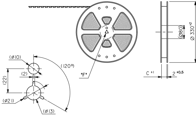
DETAIL "F"
