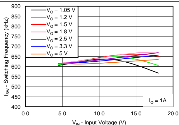
Figure 13. Switching Frequency vs Input Voltage
