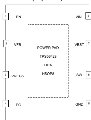
8-Pin HSOP with Thermal Pad DDA PACKAGE (Top View)
