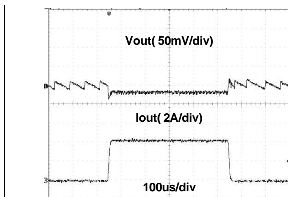
Figure 9. 1.05 V Load Transient Response
