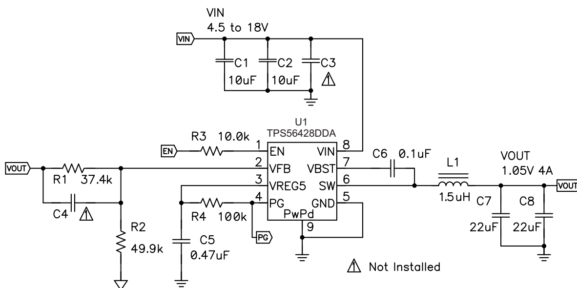
Figure 8. Schematic Diagram for This Design Example.
