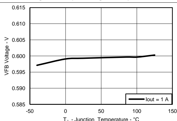
Figure 6. VFB Voltage vs Junction Temperature
