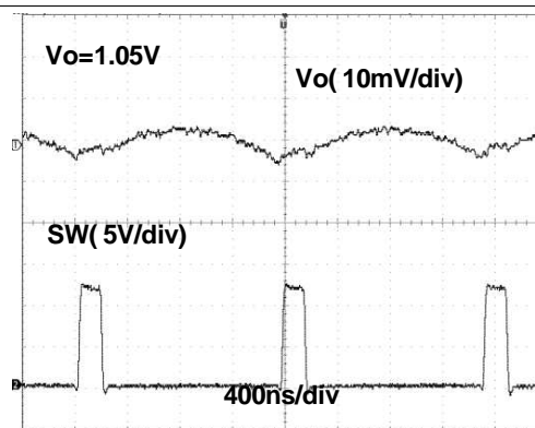
Figure 16. VOUT Ripple
