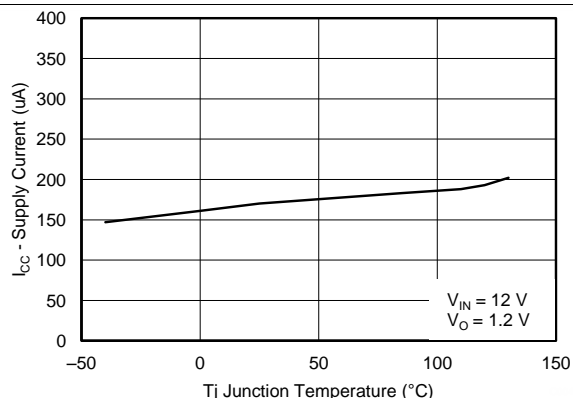
Figure 1. Supply Current vs Junction Temperature
