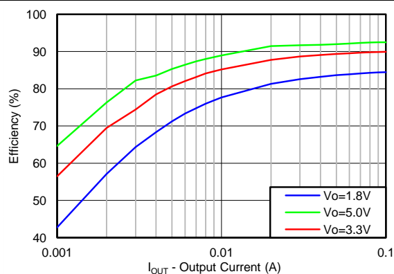
Figure 12. Efficiency vs Output Current
