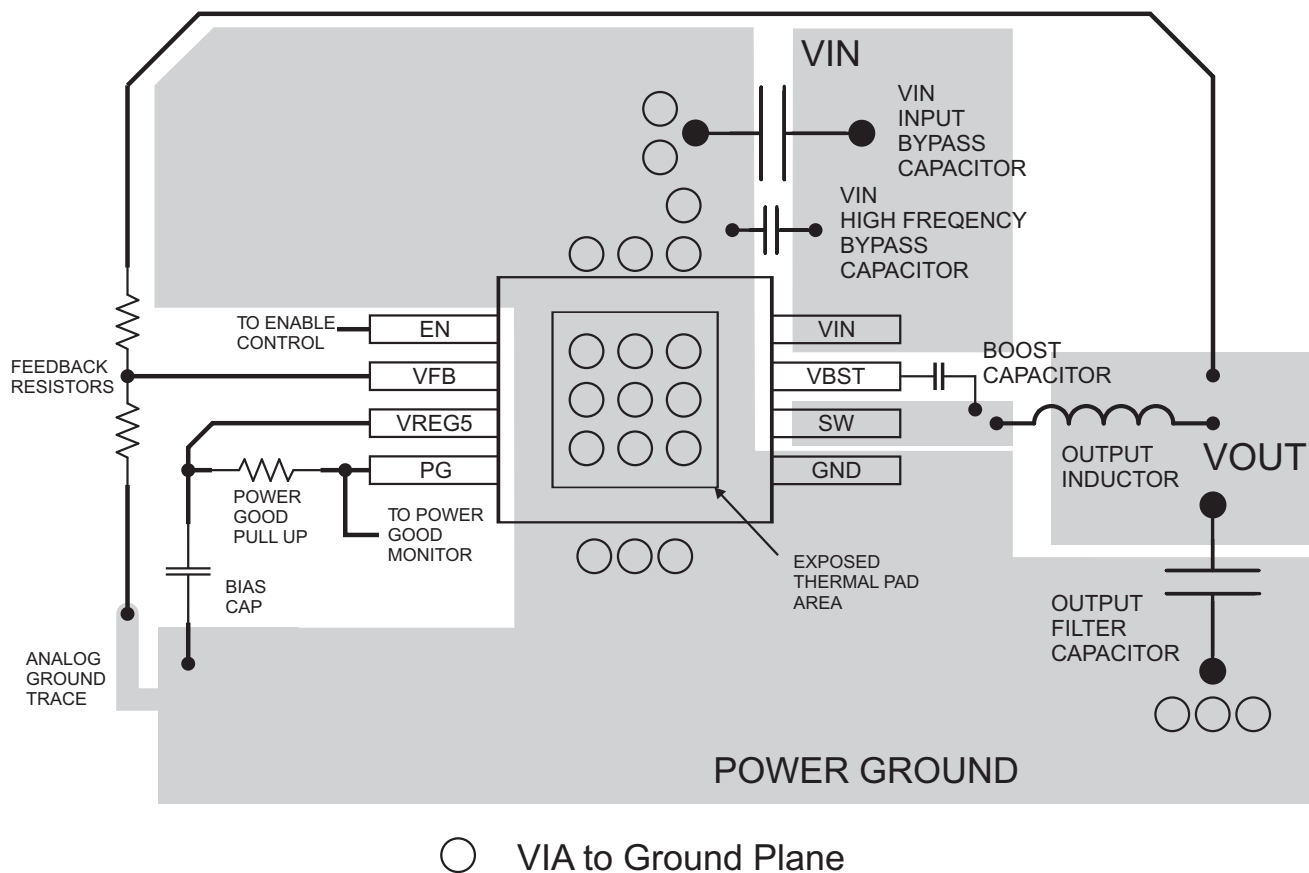
Figure 17. TPS56428 Layout – HSOP (DDA) Package
