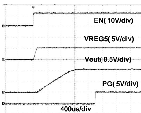
Figure 10. Slow Start
