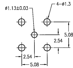
PCB MOUNTING HOLE
