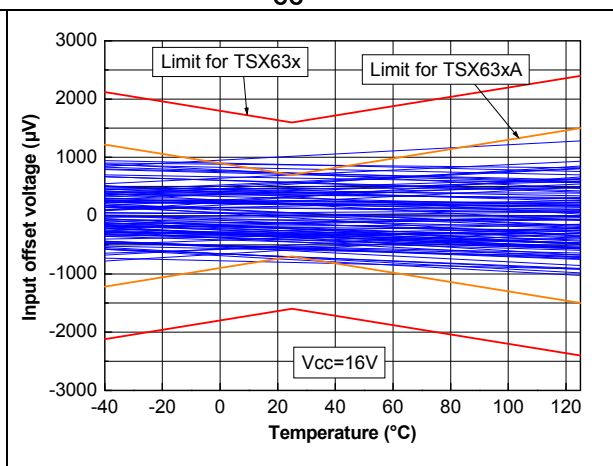
Figure 5. Input offset voltage vs. temperature at V_{CC}=16\text{ V}
