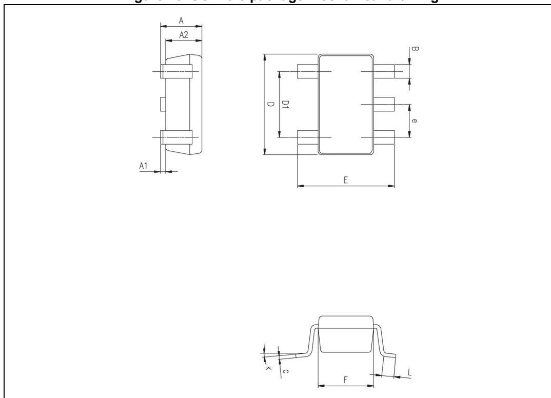
Figure 28. SOT23-5 package mechanical drawing
