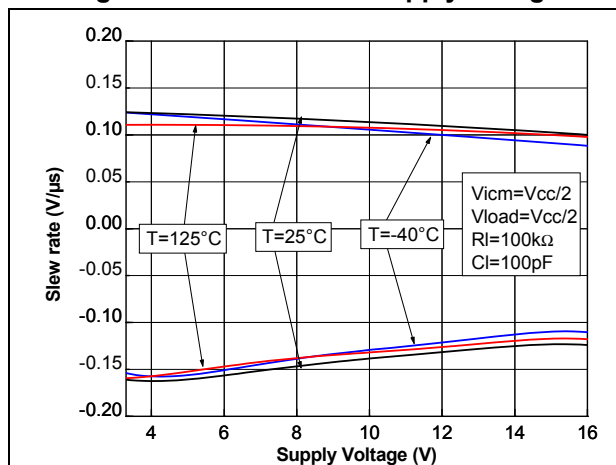
Figure 20. Slew rate vs. supply voltage
