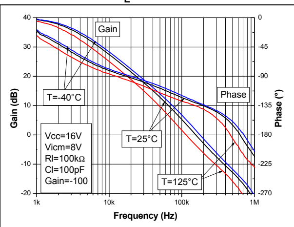
Figure 15. Bode diagram at V_{CC} = 16\text{ V} , R_L = 100\text{ k}\Omega
