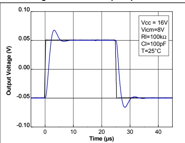
Figure 21. Small step response
