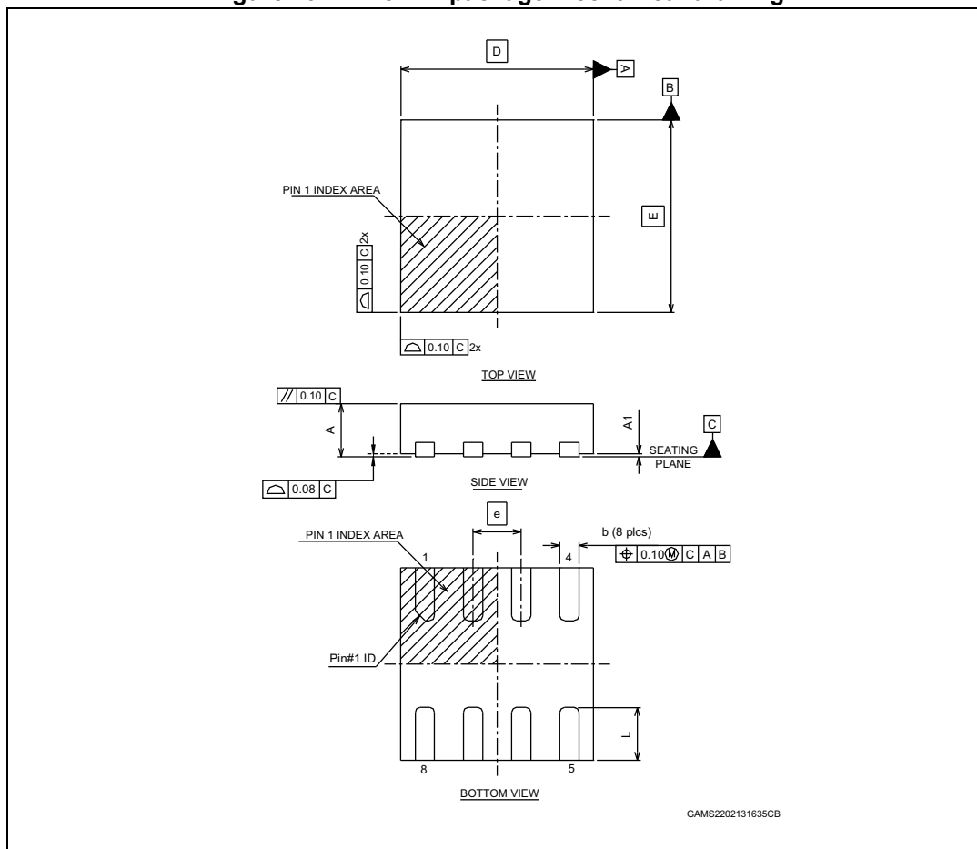
Figure 29. DFN8 2x2 package mechanical drawing
