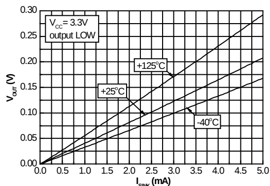
Figure 8: Output voltage vs. sink current, V_{CC} = 3.3\text{ V}
