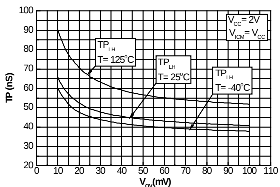
Figure 17: Propagation delay (LH) vs. overdrive at V_{CC} = 2V , V_{CM} = V_{CC}
