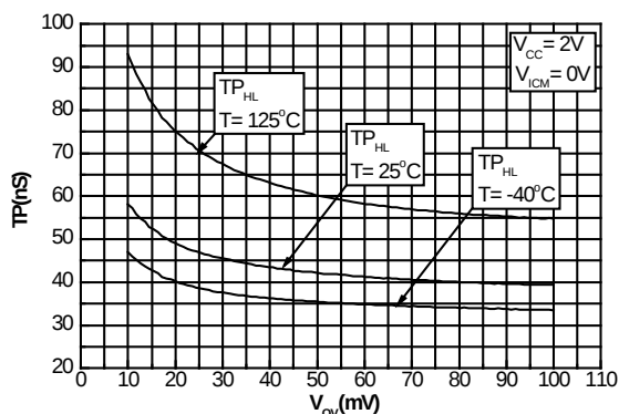
Figure 14: Propagation delay (HL) vs. overdrive at V_{CC} = 2V , V_{CM} = 0V
