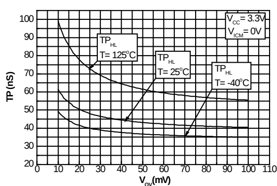
Figure 18: Propagation delay (HL) vs. overdrive at V_{CC} = 3.3V , V_{CM} = 0V
