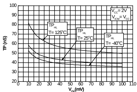
Figure 15: Propagation delay (HL) vs. overdrive at V_{CC} = 2V , V_{CM} = V_{CC}
