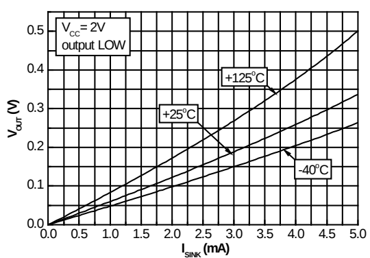
Figure 6: Output voltage vs. sink current, V_{CC} = 2V
