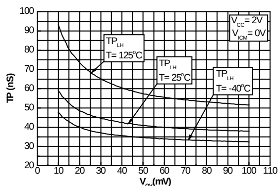
Figure 16: Propagation delay (LH) vs. overdrive at V_{CC} = 2V , V_{CM} = 0V
