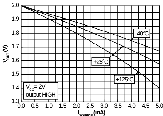
Figure 5: Output voltage vs. source current, V_{CC} = 2V
