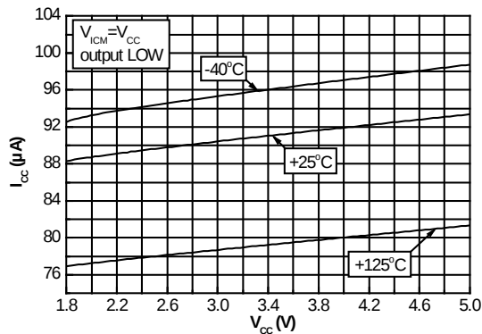
Figure 4: Current consumption vs. supply voltage ( V_{ICM} = V_{CC} , output low)
