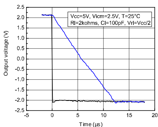
Figure 9: Negative slew rate vs. time
