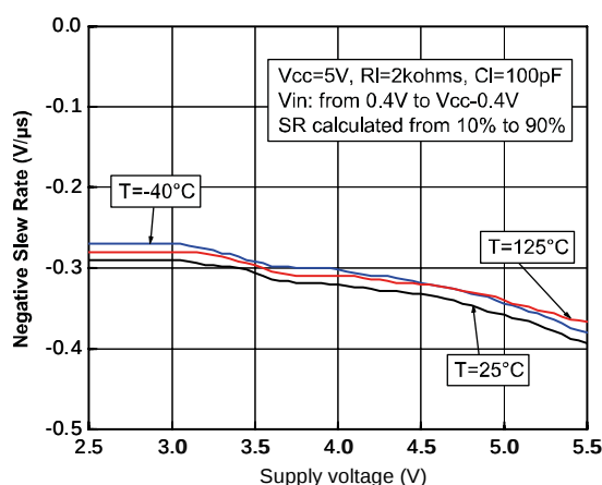
Figure 11: Negative slew rate vs. supply voltage
