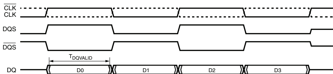
Figure 3: DDR Input Timing Diagram
