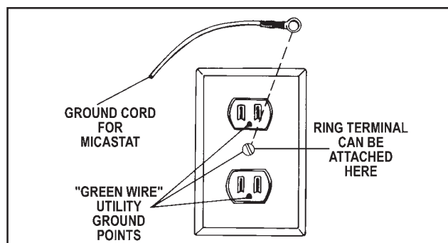
Figure 5. Outlet plate with "green wire" ground
