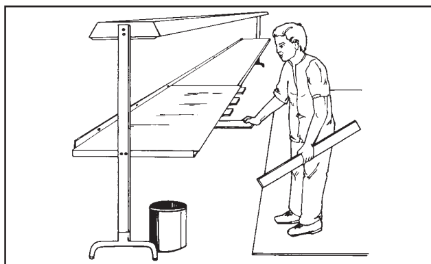
Figure 3. Micastat® sheet on wooden strips
