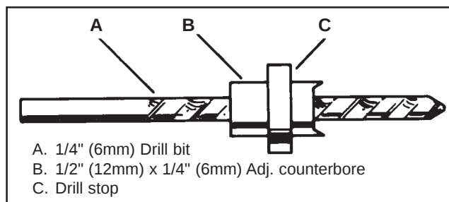
Figure 8. Drill Tool 14242.
