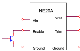
Figure 19: Enable Input drive circuit for NE series
