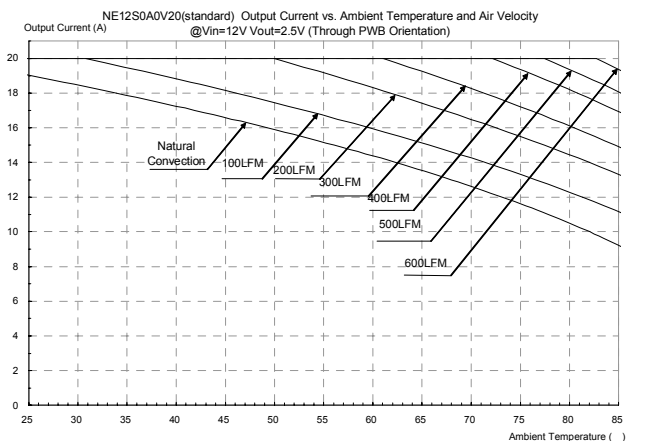
Figure 27: Output current vs. ambient temperature and air velocity @ Vin=12V, Vout=2.5V (Through PWB Orientation)
