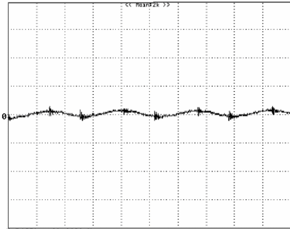
Figure 12: Input reflected ripple current, i_s , through a 12\mu\text{H} source inductor at nominal input voltage and rated load current (20 mA/div, 1 \mu\text{s} /div)
