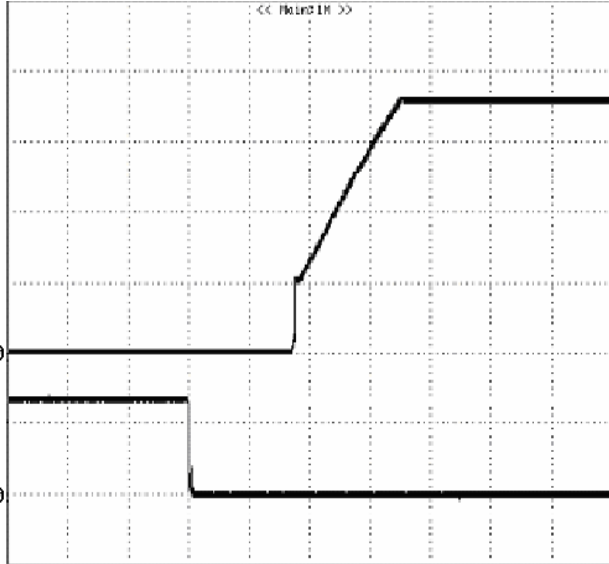
Figure 4: Turn-on transient at full rated load current (resistive load) (5 ms/div). V_{in}=48V . Top Trace: V_{out} , 0.5V/div; Bottom Trace: ON/OFF input, 2V/div
