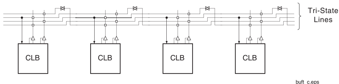
Figure 8: BUFT Connections to Dedicated Horizontal Bus Lines
