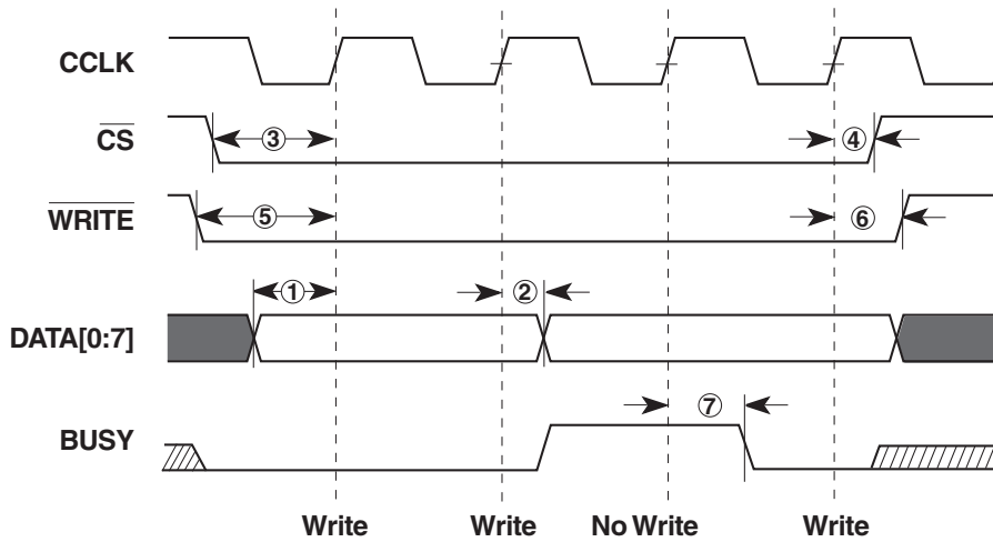
Figure 16: Write Operations
