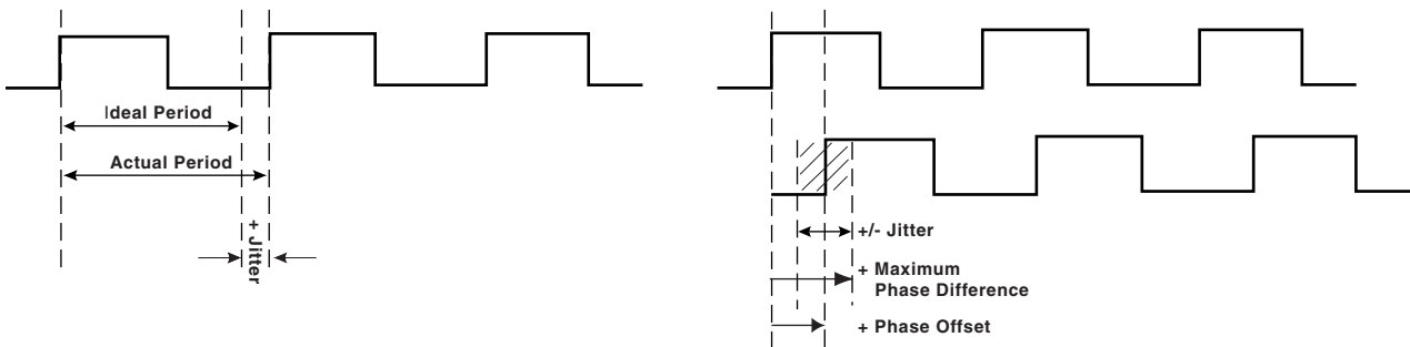
Figure 1: Frequency Tolerance and Clock Jitter
