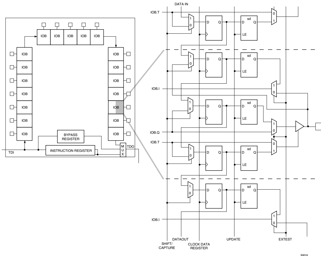
Figure 10: Virtex Series Boundary Scan Logic
