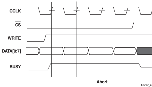
Figure 18: SelectMAP Write Abort Waveforms
