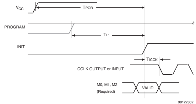
Figure 19: Power-Up Timing Configuration Signals
