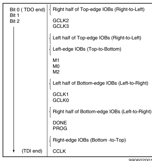
Figure 11: Boundary Scan Bit Sequence
