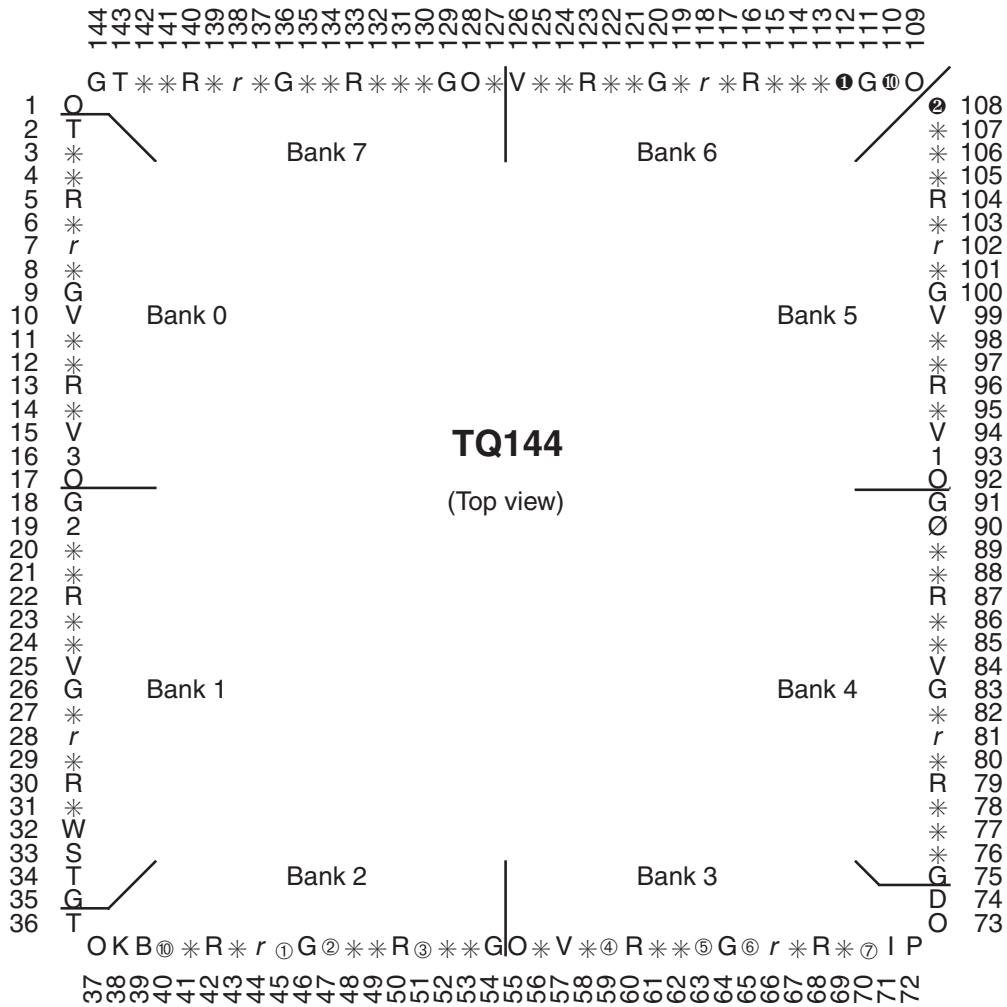
Figure 2: TQ144 Pin Function Diagram
