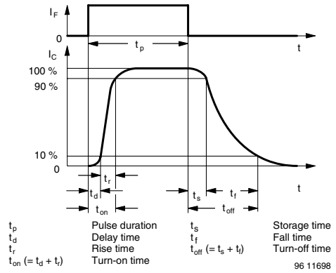
Fig. 3 - Switching Times
