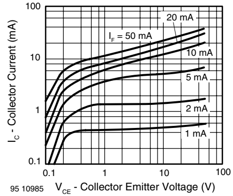
Fig. 9 - Collector Current vs. Collector Emitter Voltage
