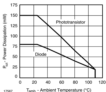
Fig. 1 - Permissible Power Dissipation vs. Temperature
