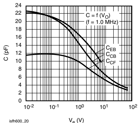
Fig. 20 - Transistor Capacitance
