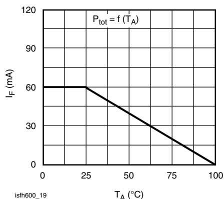
Fig. 19 - Permissible Forward Current Diode
