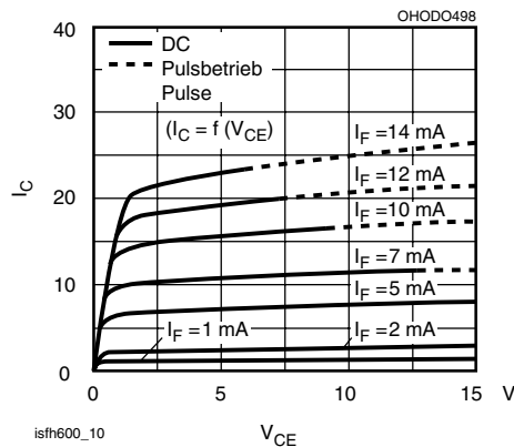
Fig. 10 - Output Characteristics SFH600-2, -3
