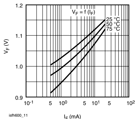
Fig. 11 - Forward Voltage
