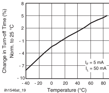
Fig. 19 - Turn-off Time vs. Temperature
