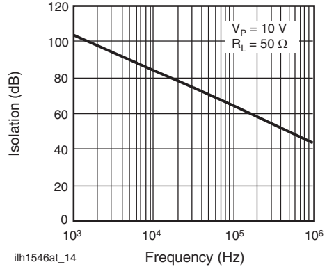
Fig. 14 - Output Isolation
