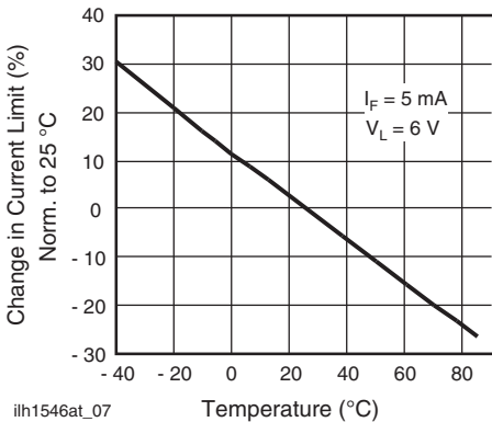
Fig. 7 - Current Limit vs. Temperature
