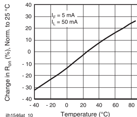
Fig. 10 - On-resistance vs. Temperature
