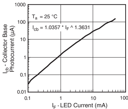
Fig. 9 - Collector Base Photocurrent vs. LED Current
