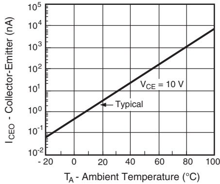
Fig. 7 - Collector Emitter Leakage Current vs. Temperature
