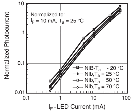
Fig. 10 - Normalized Photocurrent vs. I_F and Temperature
