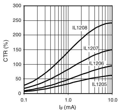
Fig. 10 - CTR vs. I_F , ( V_{CE} = 5\text{ V} , T_{amb} = 25\text{ °C} ) (Not Normalised)
