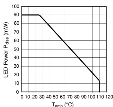
Fig. 1 - Input Power Dissipation (LED) vs. Ambient Temperature
