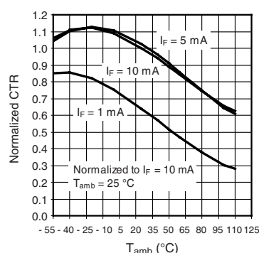
Fig. 8 - CTR Normalized to I_F = 10\text{ mA} vs. Ambient Temperature, (Saturated, V_{CE} = 0.4\text{ V} )
