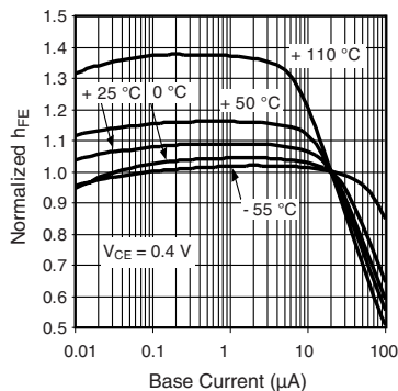
Fig. 15 - Normalized h_{FE} vs. Base Current and T_{amb} (Saturated Condition)
