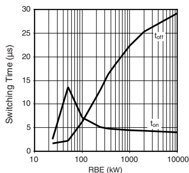
Fig. 21 - Switching Time vs. RBE, I_F = 10 mA
