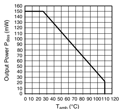
Fig. 2 - Output Power Dissipation vs. Ambient Temperature
