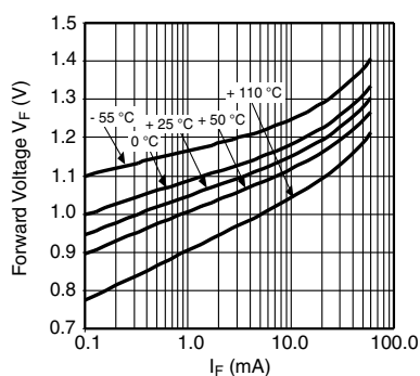
Fig. 4 - Diode Forward Voltage V_F vs. Forward Current
