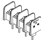
AUX. VIEW SCALE 1:1 (4 CIRCUIT SHOWN)
