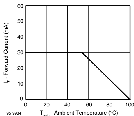
Fig. 2 - Forward Current vs. Ambient Temperature for InGaAl
