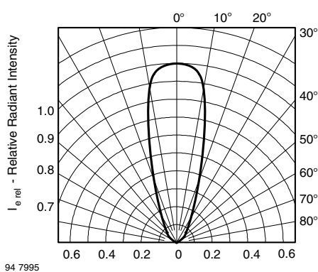
Fig. 9 - Relative Radiant Intensity vs. Angular Displacement
