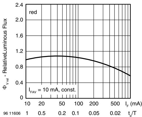
Fig. 5 - Relative Luminous Flux vs. Forward Current/Duty Cycle
