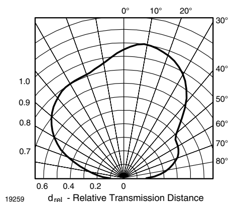
Fig. 4 - Vertical Directivity
