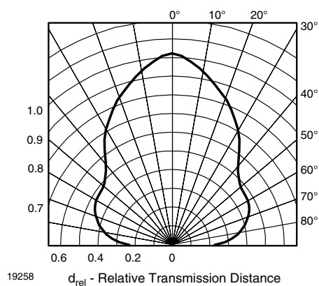
Fig. 3 - Horizontal Directivity
