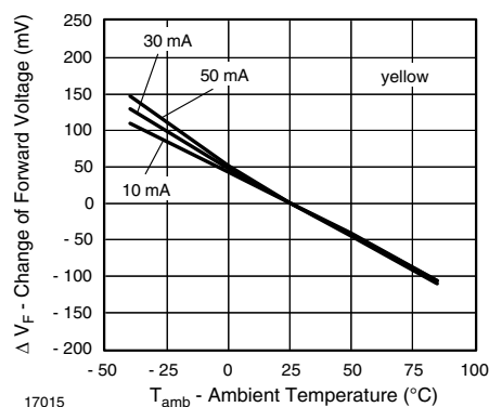
Fig. 20 - Change of Forward Voltage vs. Ambient Temperature
