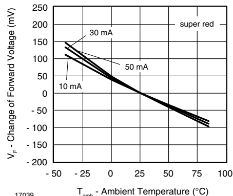
Fig. 8 - Change of Forward Voltage vs. Ambient Temperature
