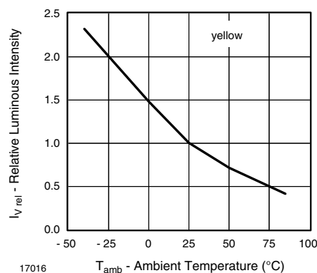
Fig. 18 - Relative Luminous Intensity vs. Ambient Temperature
