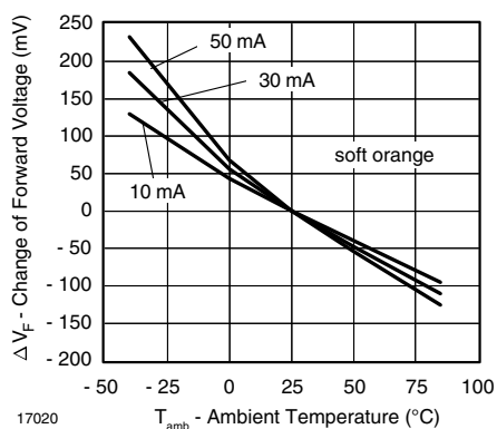
Fig. 16 - Change of Forward Voltage vs. Ambient Temperature
