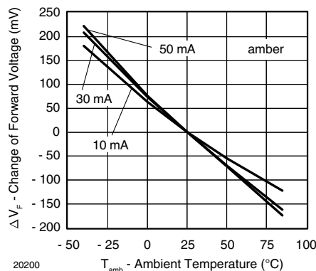
Fig. 12 - Change of Forward Voltage vs. Ambient Temperature
