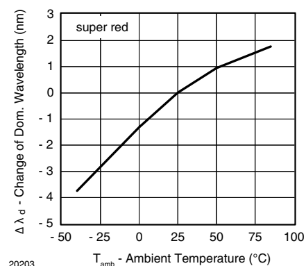
Fig. 7 - Change of Dominant Wavelength vs. Ambient Temperature
