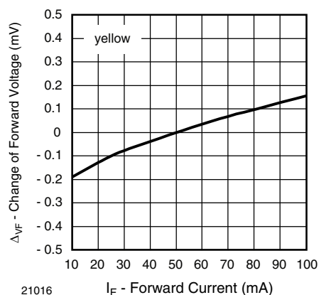
Fig. 5 - Change of Forward Voltage vs. Forward Current
