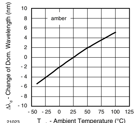
Fig. 12 - Change of Dominant Wavelength vs. Ambient Temperature
