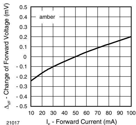
Fig. 6 - Change of Forward Voltage vs. Forward Current
