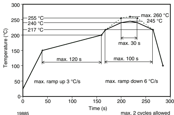
Fig. 15 - Vishay Lead (Pb)-free Reflow Soldering Profile (according to J-STD-020B)
