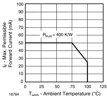
Fig. 1 - Maximum Permissible Forward Current vs. Ambient Temperature
