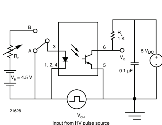
Fig. 3 - Test Circuit for Common Mode Transient Immunity
