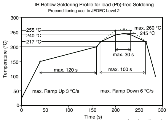
19470-4 max. 2 cycles allowed Fig. 9 - Vishay Lead (Pb)-free Reflow Soldering Profile (acc. to J-STD-020)
