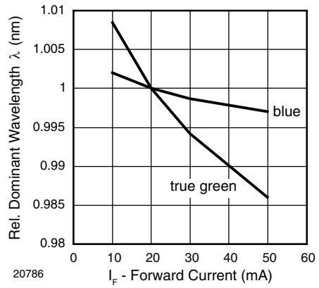
Fig. 6 - Relative Dominant Wavelength vs. Forward Current
