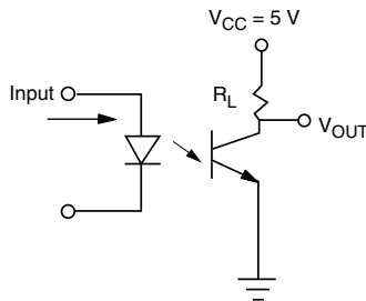
Fig. 4 - Test Circuit
