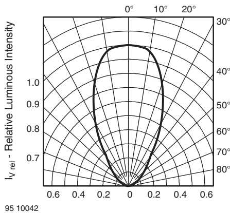
Fig. 3 - Rel. Luminous Intensity vs. Angular Displacement
