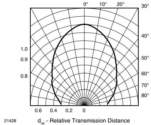
Fig. 12 - Vertical Directivity
