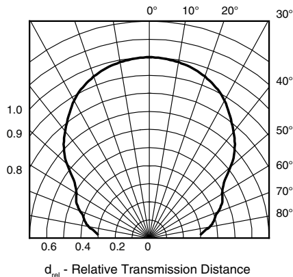
Fig. 11 - Horizontal Directivity
