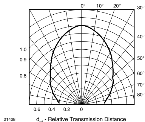
Fig. 12 - Vertical Directivity
