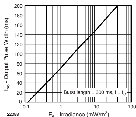
Fig. 8 - Output Pulse Width vs. Irradiance
