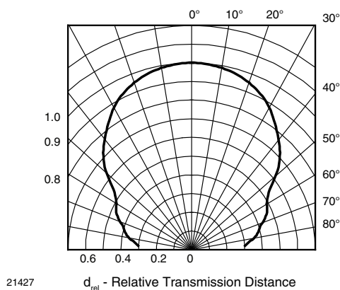
Fig. 11 - Horizontal Directivity
