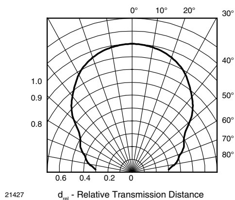
Fig. 3 - Horizontal Directivity
