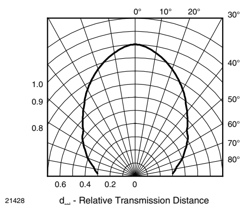
Fig. 4 - Vertical Directivity
