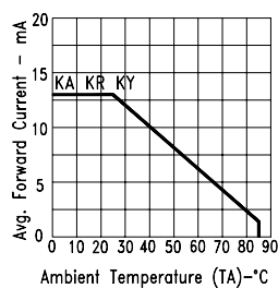
Fig. 4. Max. Average Forward Current vs. Ambient Temperature.
