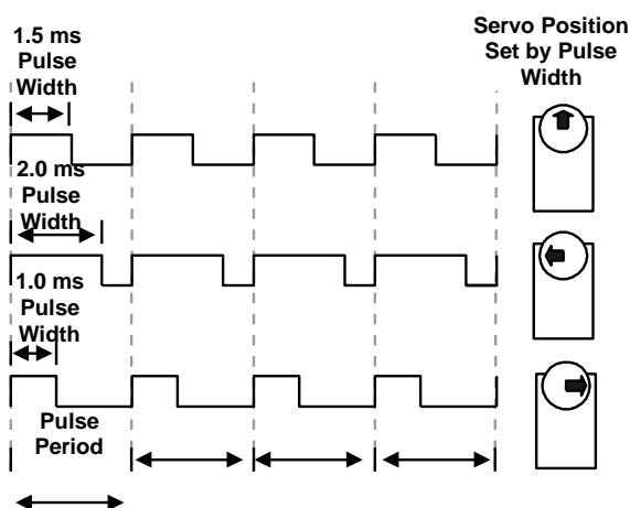
Figure 1. Servo control diagram.
