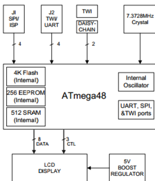
Figure 1. PmodCLS block diagram.
