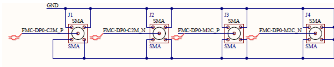
Figure 6. SMA Schematics
