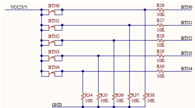
Figure 4. Schematic for Buttons
