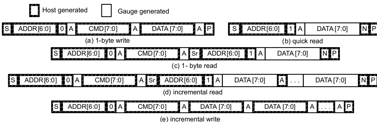
Figure 7. I 2 C Read, Incremental Read, Quick Read, One Byte Write, and Incremental Write Functions
