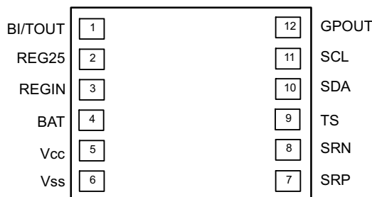
DRZ Package 12-Pin SON Top View
