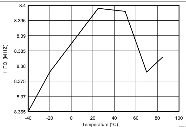
Figure 14. High Frequency Oscillator vs. Temperature
