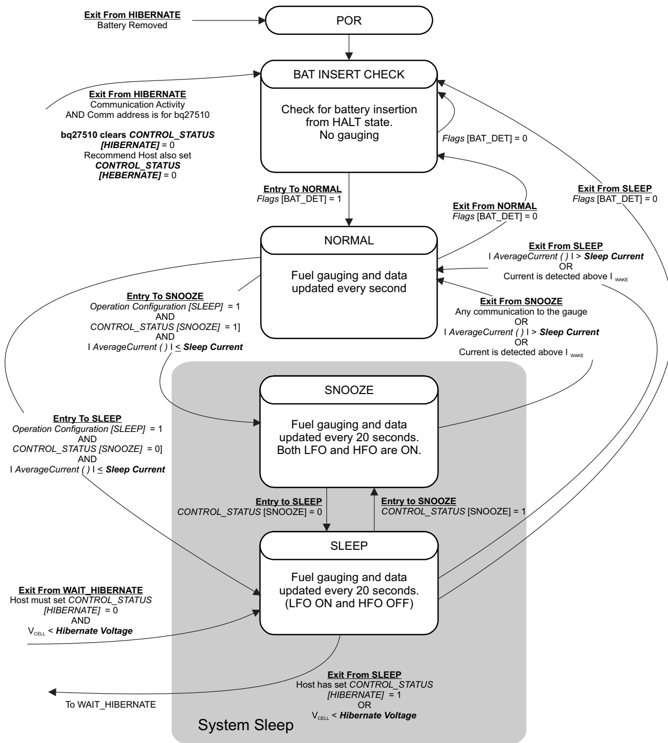
Figure 6. Power Mode Diagram for System Sleep
