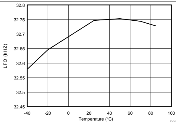
Figure 13. Low Frequency Oscillator vs. Temperature
