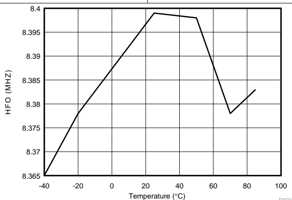
Figure 4. High Frequency Oscillator vs. Temperature
