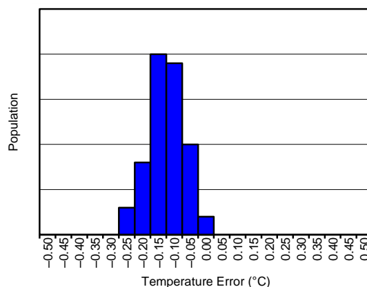
Figure 6. TEMPERATURE ERROR AT +25^\circ\text{C}
