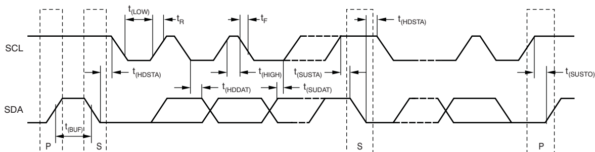
Figure 12. Two-Wire Timing Diagram
