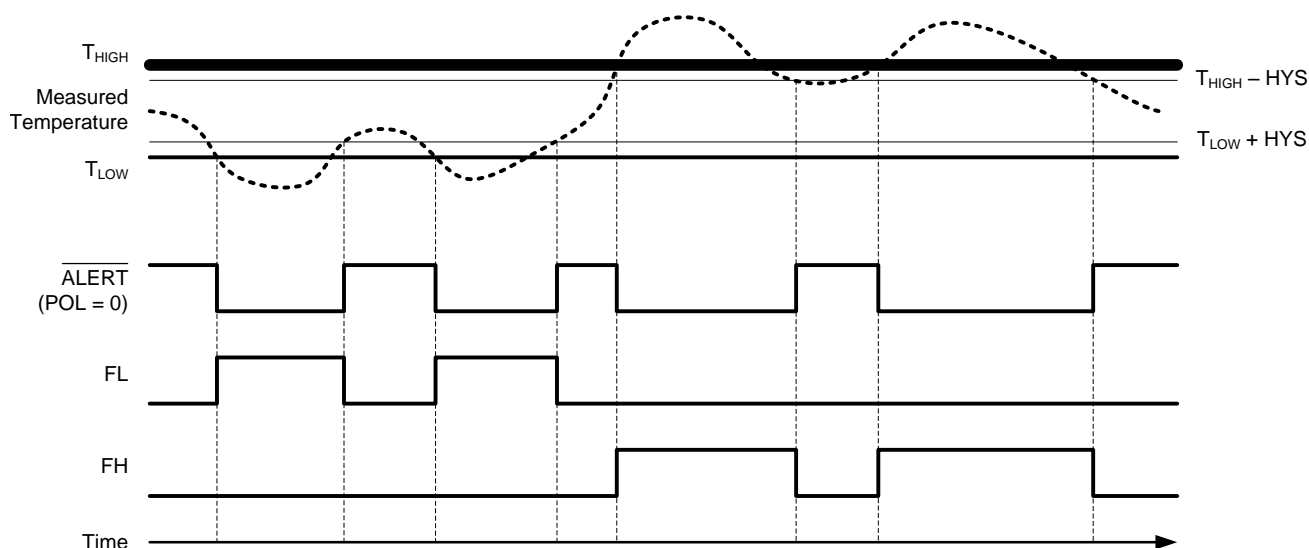
Figure 11. Comparator Mode
