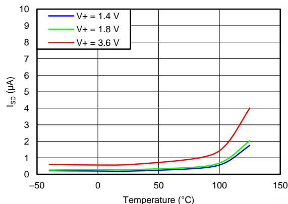
Figure 2. SHUTDOWN CURRENT vs TEMPERATURE
