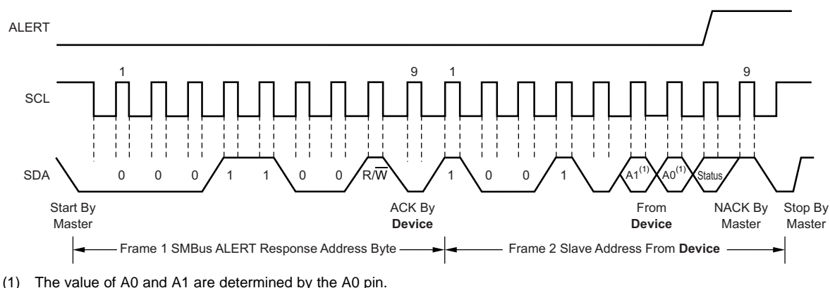
Figure 15. Timing Diagram for SMBus Alert
