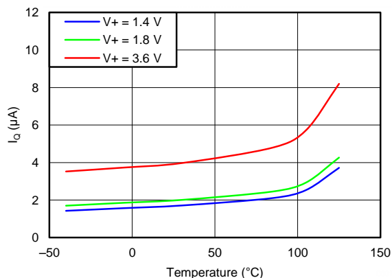
Figure 1. QUIESCENT CURRENT vs TEMPERATURE (1 Conversion per Second)
