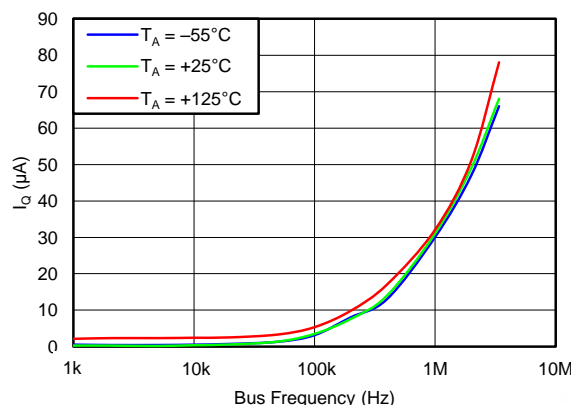
Figure 4. QUIESCENT CURRENT vs BUS FREQUENCY
