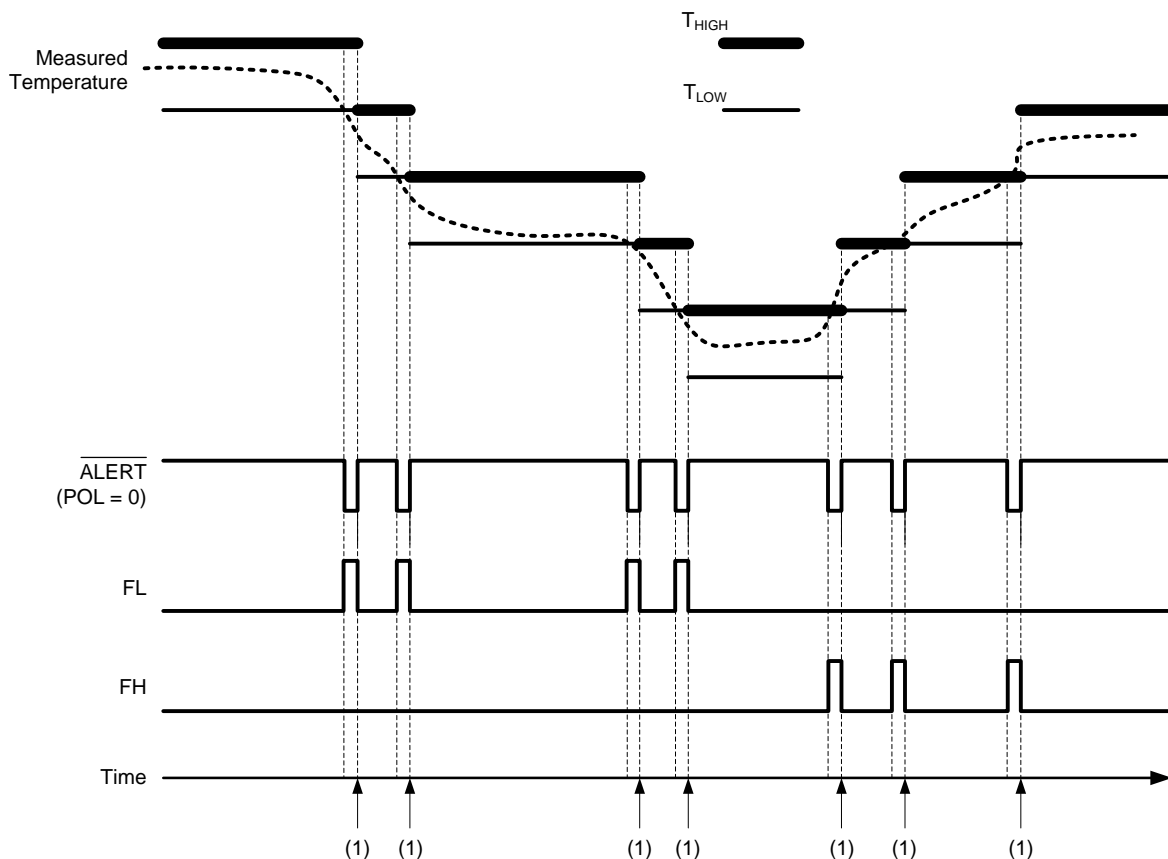
Figure 10. Interrupt Mode
