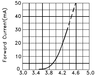
Forward Voltage(V) FORWARD CURRENT Vs FORWARD VOLTAGE
