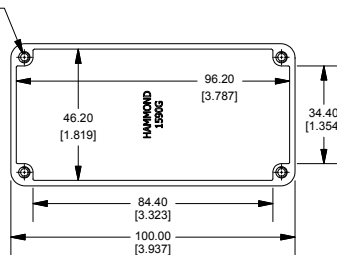
Top View Looking Inside Box
