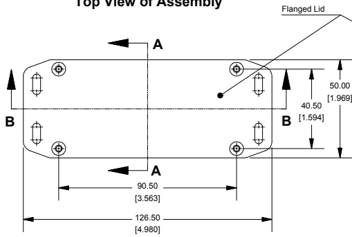
Top View of Assembly
