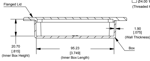
SECTION B-B Side View of Assembly
