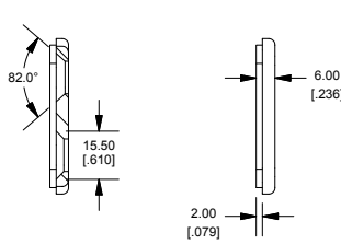
SECTION C-C Side of Slot
