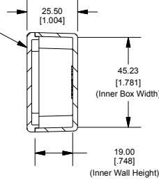
SECTION A-A End View of Assembly
