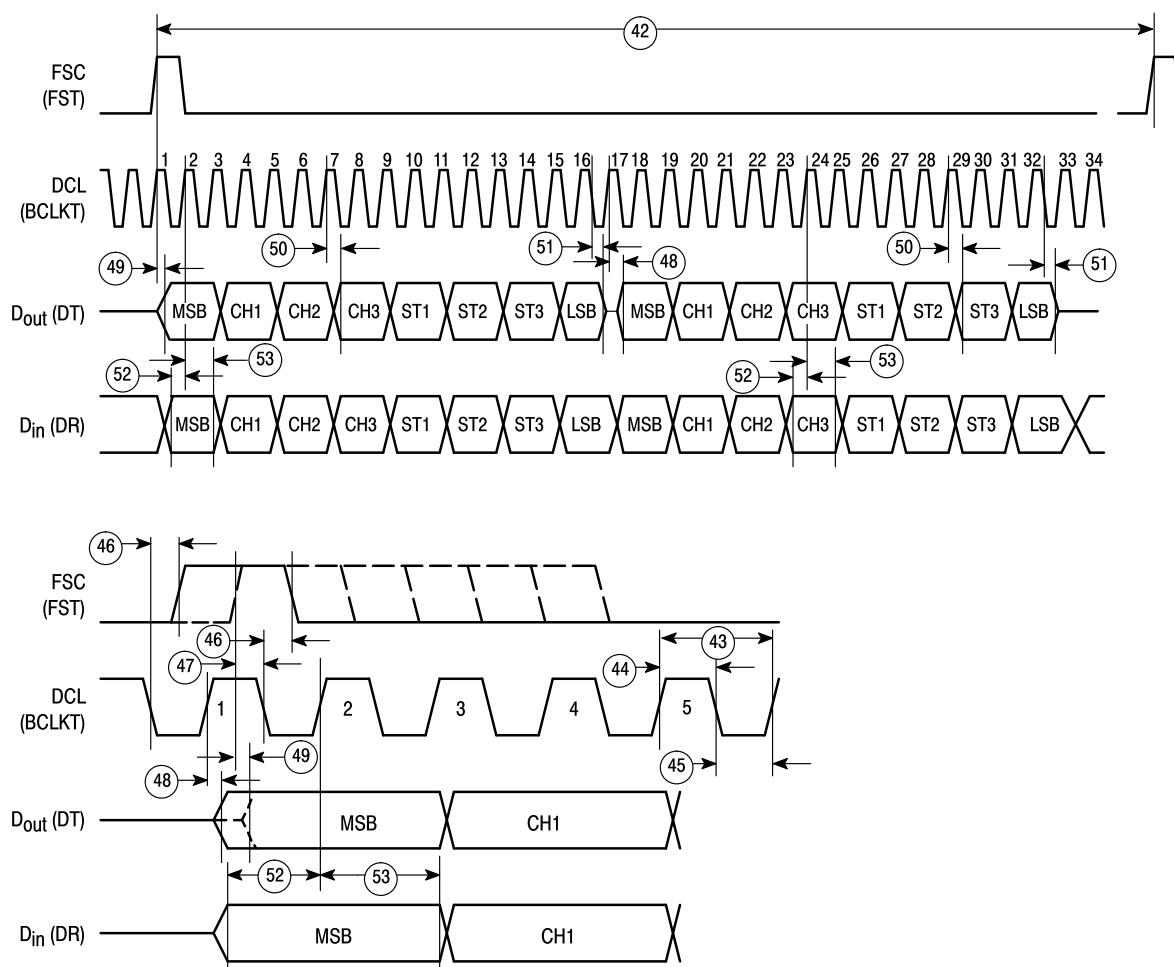
Figure 6. GCI Interface Timing
