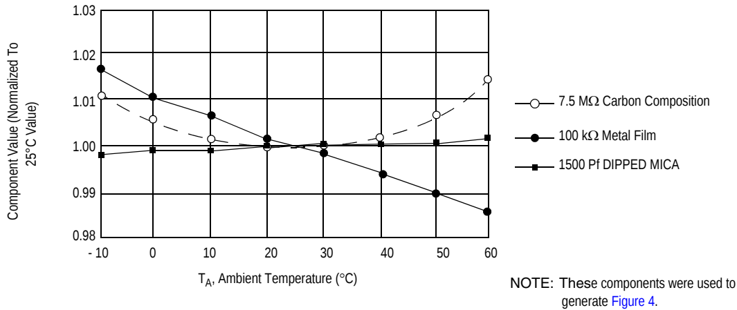
Figure 5. RC Component Variation Over Temperature
