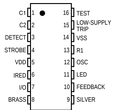
Figure 1. Pin Connections
