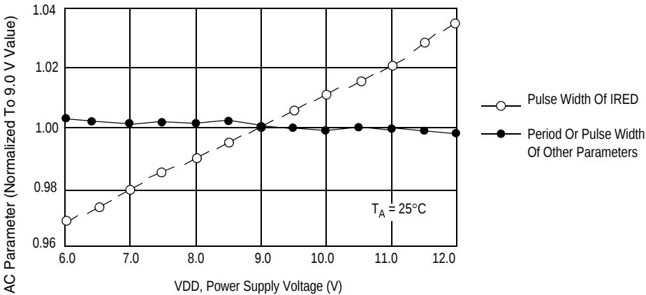
Figure 3. AC Characteristics versus Supply
